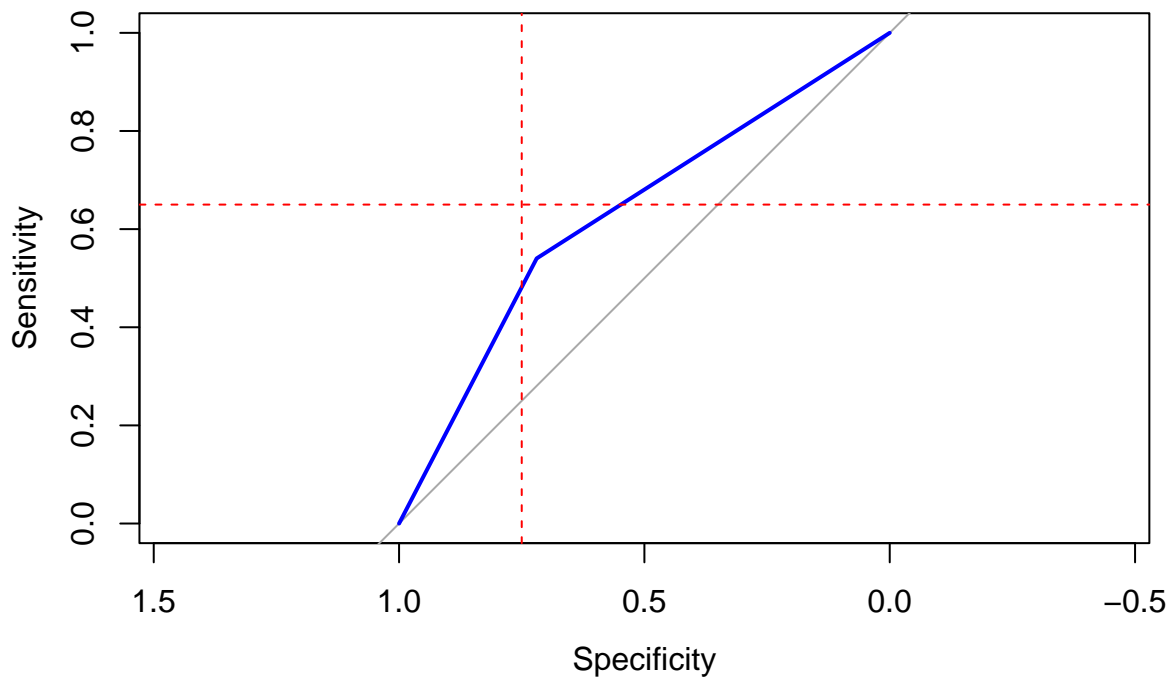
ROC: Model 2.1
