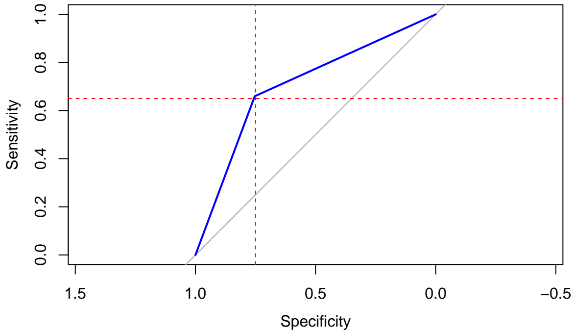
ROC: Model 1.2
