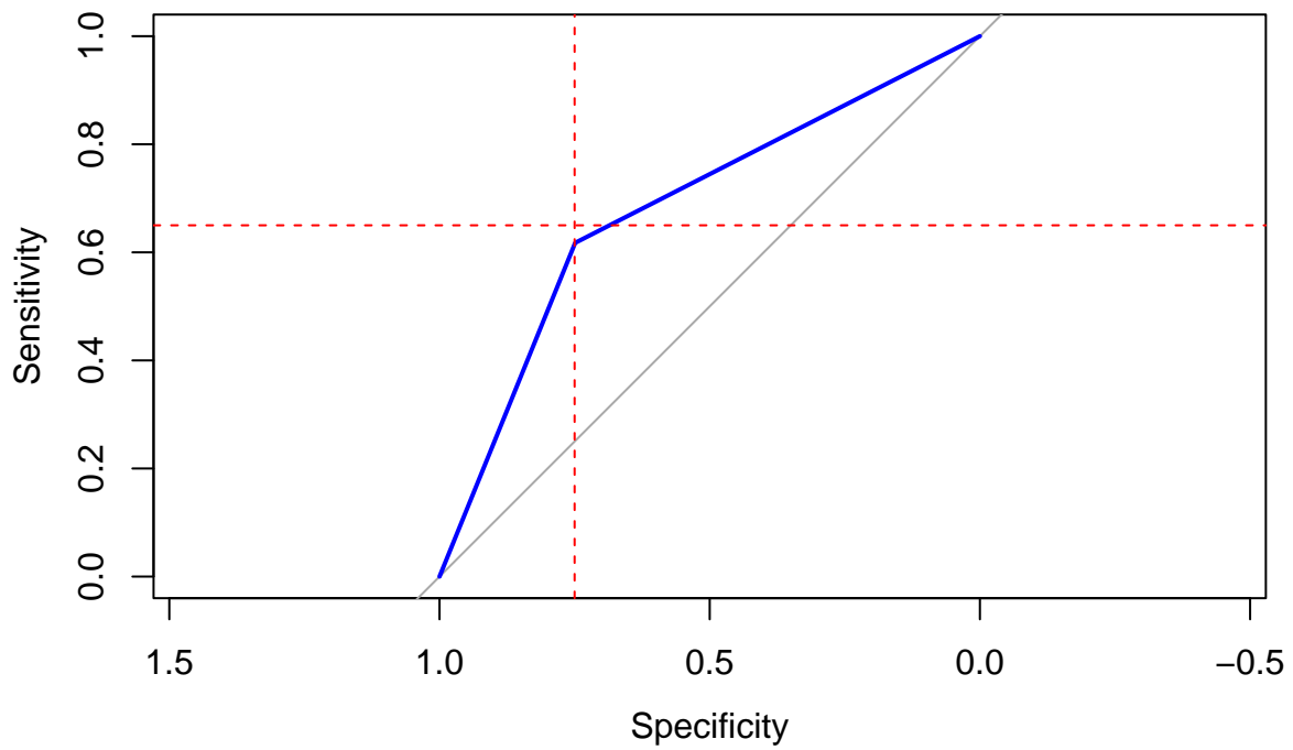
ROC: Model 3.1
