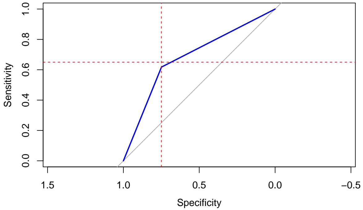
ROC: Model 2.2
