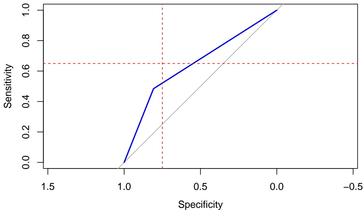
ROC: Model 6.1
