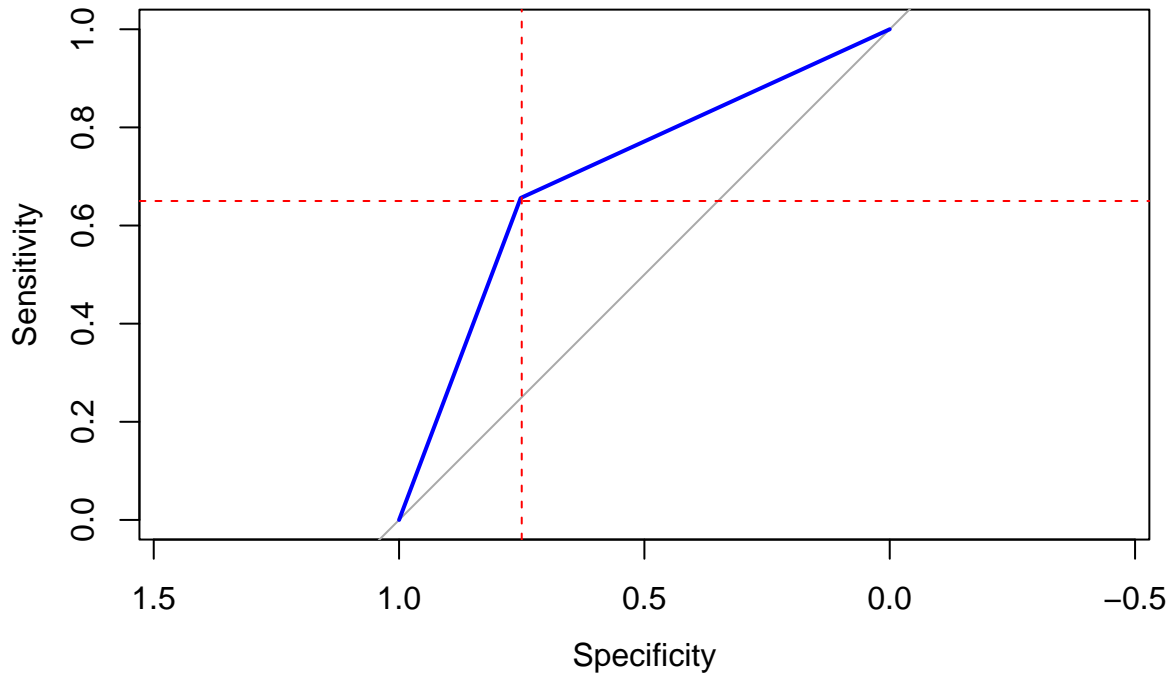
ROC: Model 4.1
